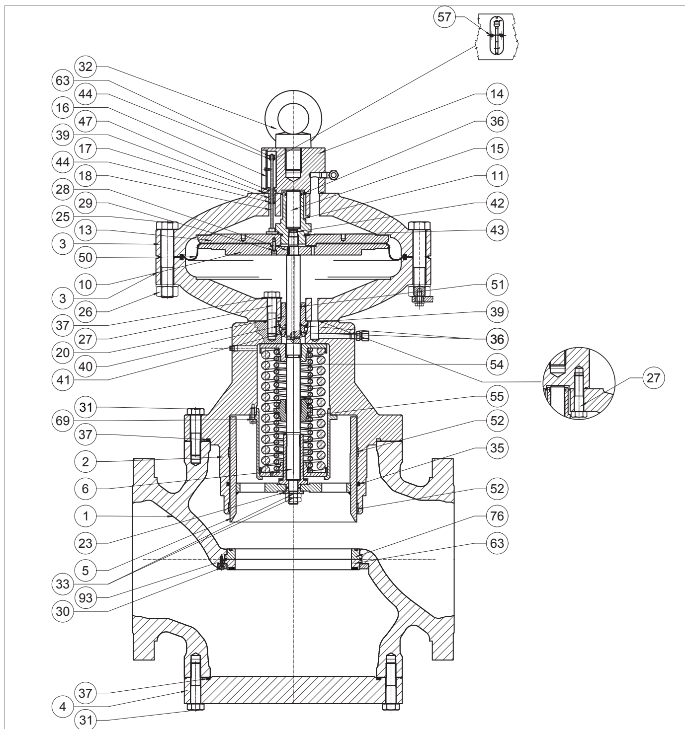
Regulator REFLEX 819/FO 10"
