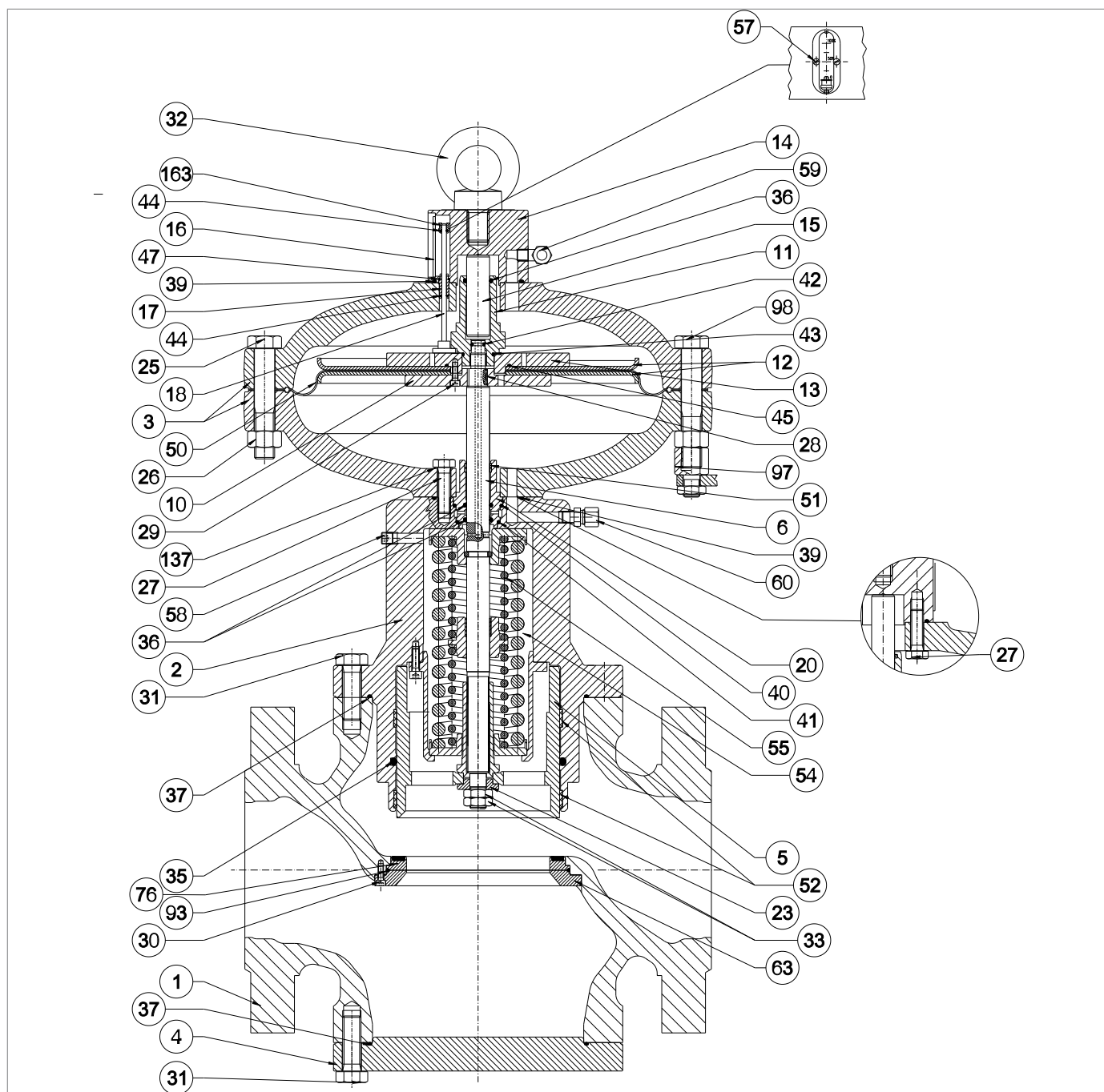
Rys. 9.57. Regulator REFLUX 819/FO 4" ÷ 8"
