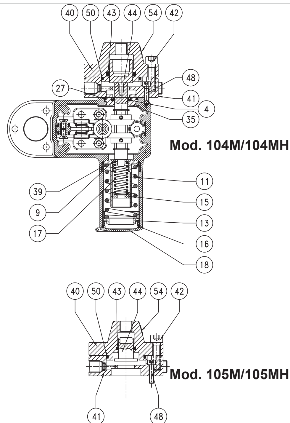
Rys. 9.77. Presostat Mod. 104M/104MH ÷ 105M/105MH
