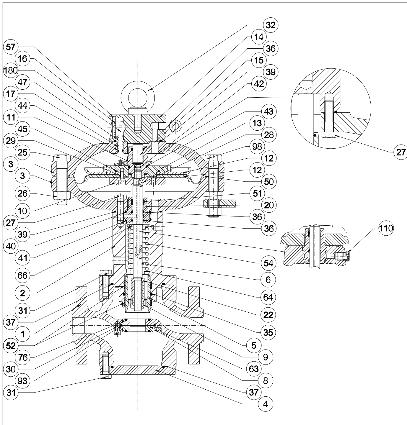
Rys. 9.55. Regulator REFLUX 819/FO 1"
