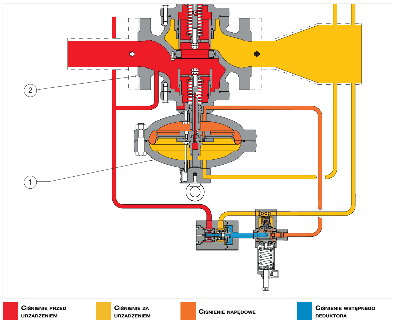
Rys. 4.5. REFLUX 819/FO z monitorem PM/819
