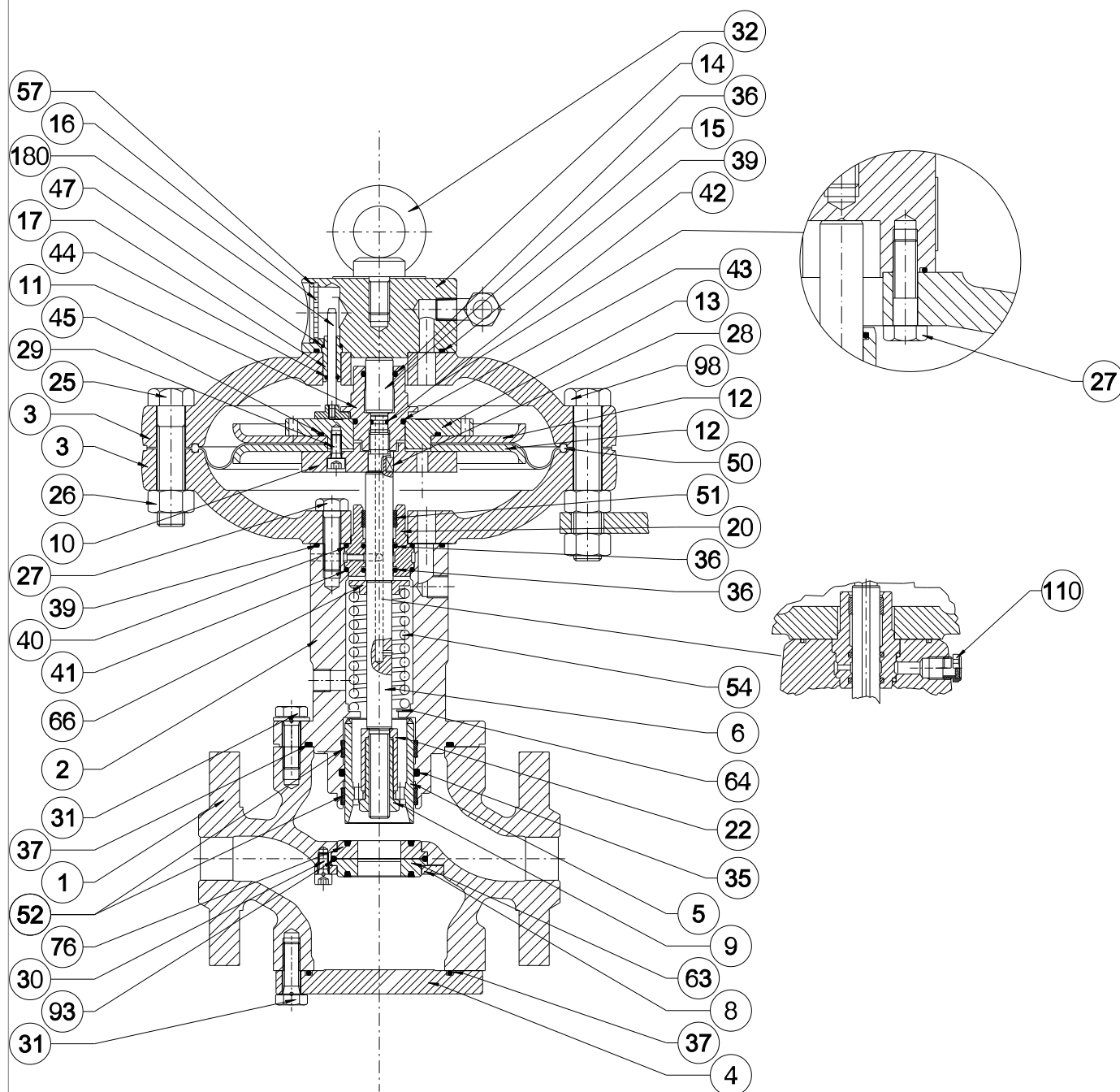
Regulator REFLEX 819/FO 1"
