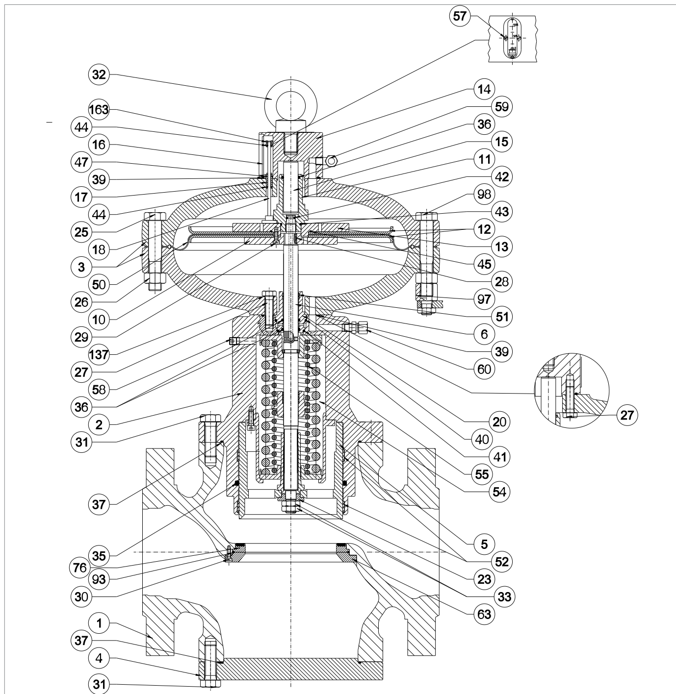
Regulator REFLEX 819/FO 4" ÷ 8"
