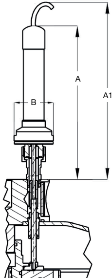
Figure 21 Q-KIT dimensions
