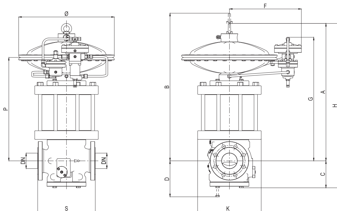
Figure 14 Dimensions Reval 182 + DB/182
