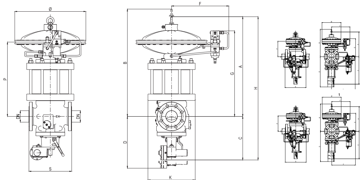
Figure 15 Dimensions Reval 182 + DB/182 + SB/82 ou HB/97
