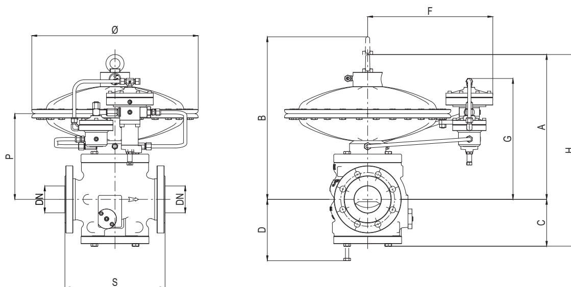
Figure 10 Dimensions Reval 182
