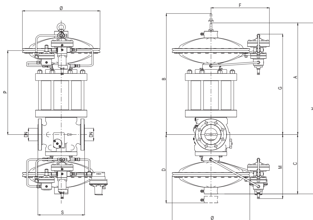
Figure 17 Dimensions Reval 182 + DB/182 + PM/182
