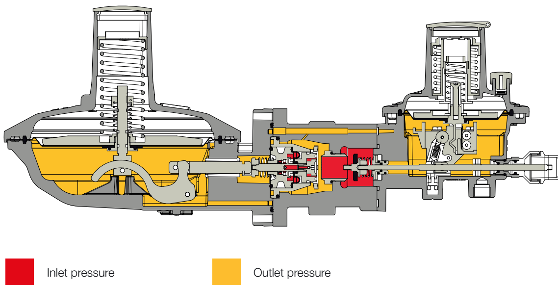
Figure 10 Dival 500 with LA
