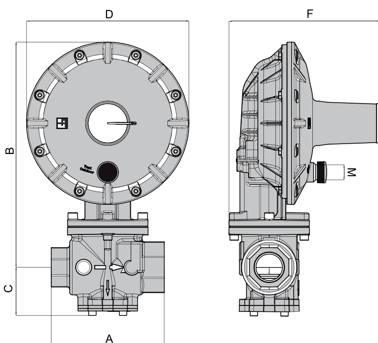
Figure 11 Dival 500 dimensions
