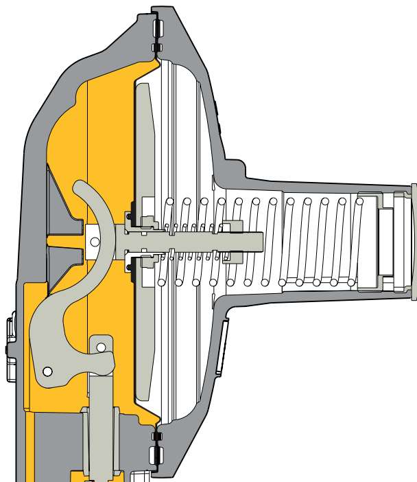
Figure 9 Dival 500 relief valve
