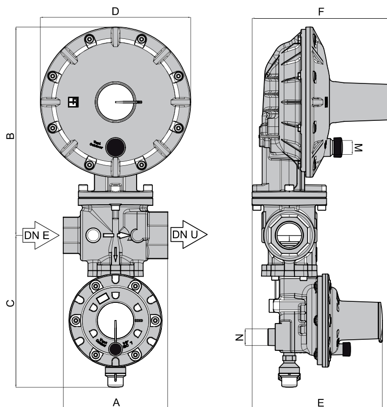
Figure 12 Dival 500 + LA dimensions
