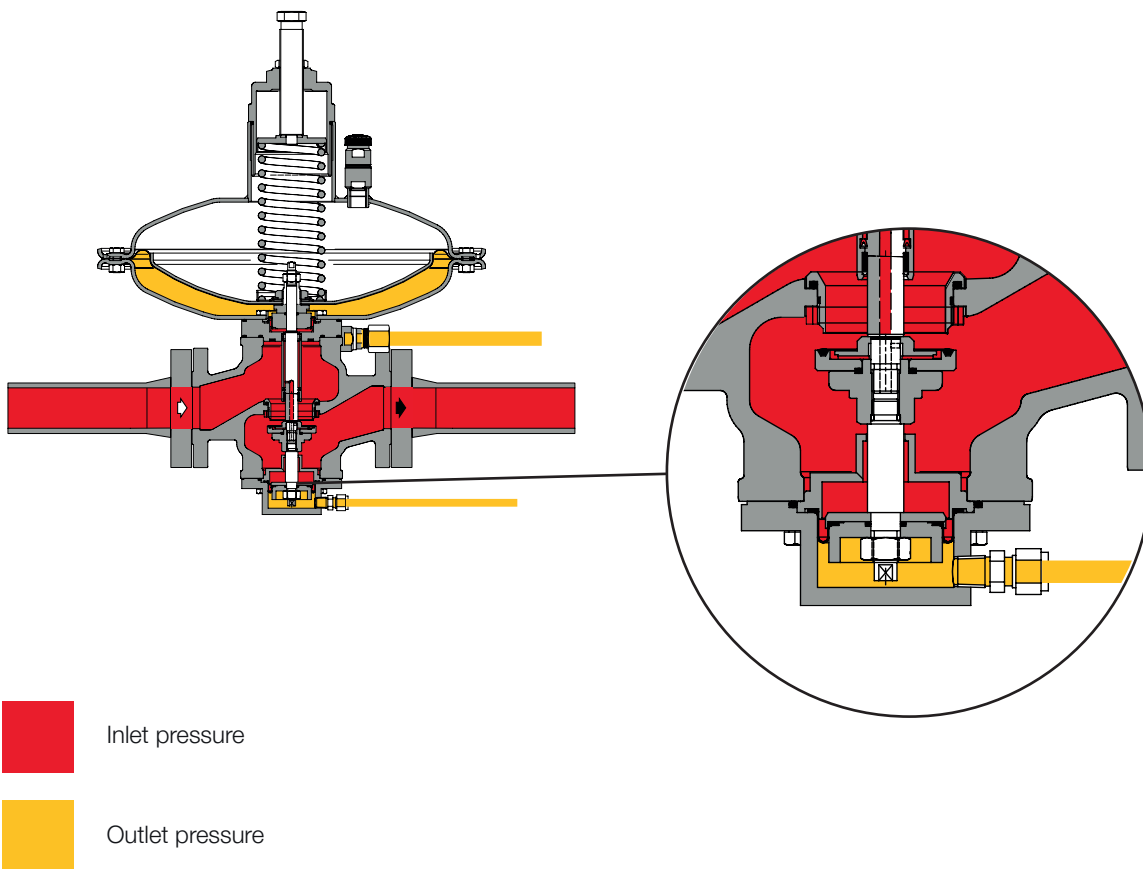
Figure 5 Norval with ER attachment
