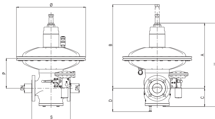
Figure 9 Norval + SN dimensions
