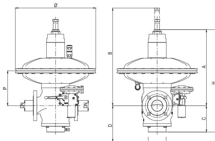
Figure 11 Norval + SN + ER attachment dimensions
