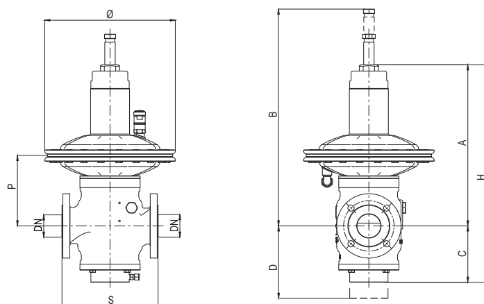
Figure 10 Norval + ER attachment dimensions
