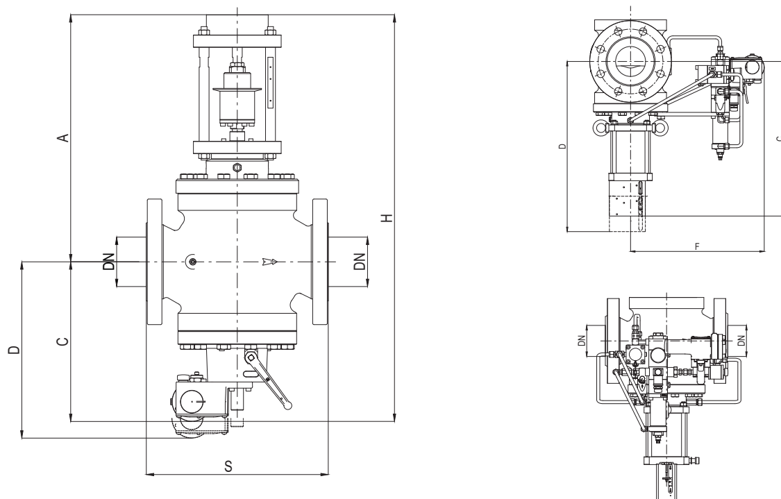
Figura 10 Syncroflux + dimensiones SB/82 o HB/97
