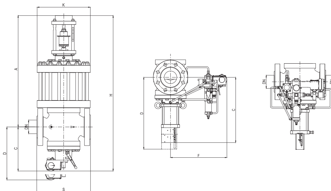
Figura 12 Dimensiones Syncroflux + DB/819 + SB/82 o HB/97
