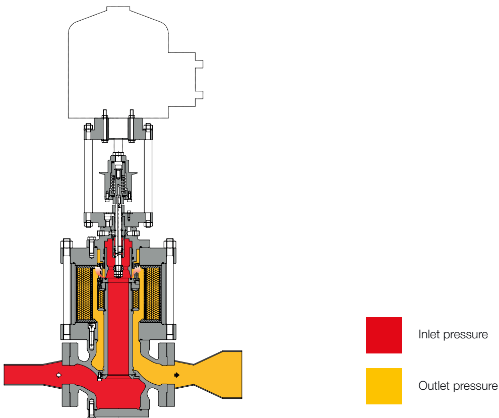
Figure 6 Syncroflux with DB/819 silencer
