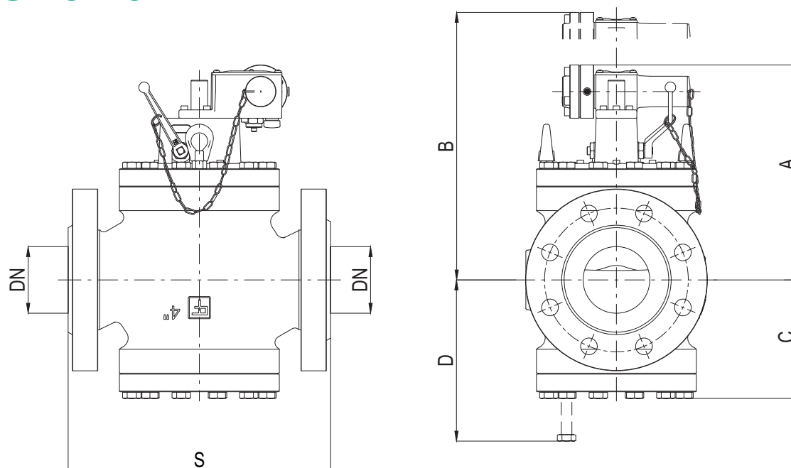
Figure 6 SBC 782 dimensions
