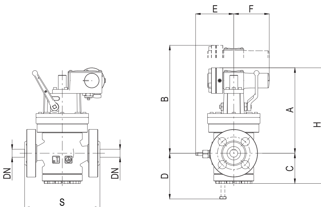
Figure 5 Dimensions SBC 187
