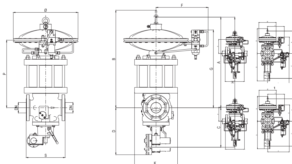
Figure 20 Reval 182 + DB/182 + SB/82 or HB/97 dimensions
