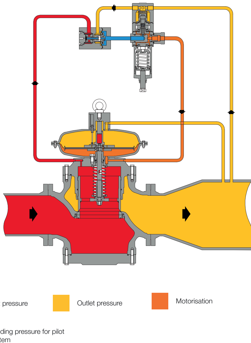
Figure 10 Reval 182 with fail to open pilot series 210
