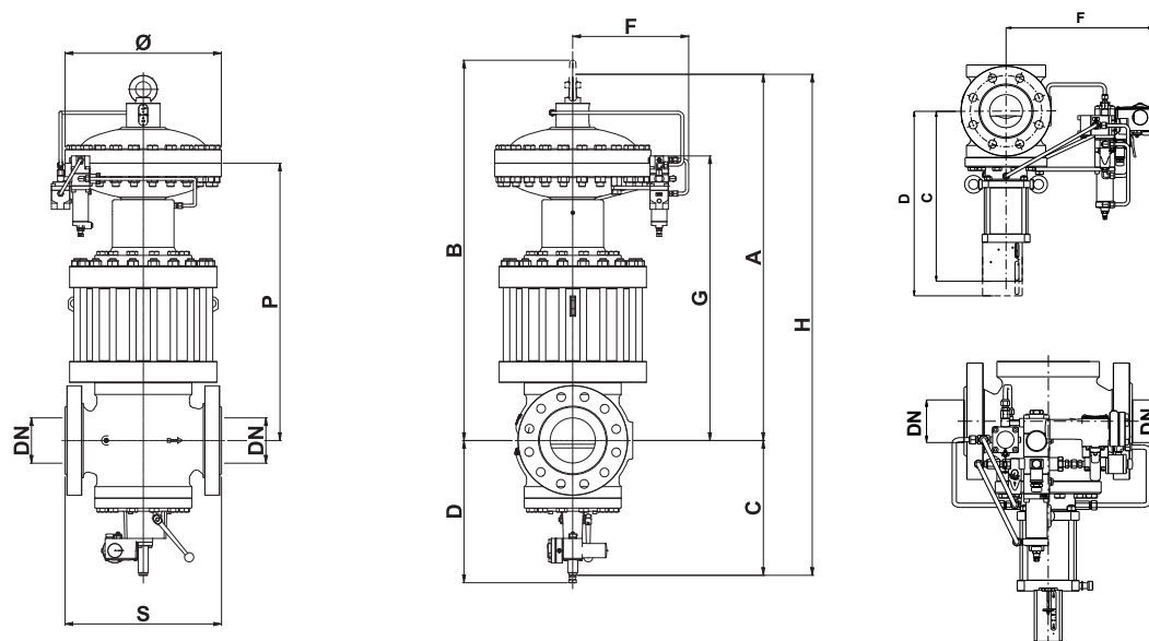
Figure 14 Reflux 819/FO + DB/819 + SB/82 or HB/97 dimensions
