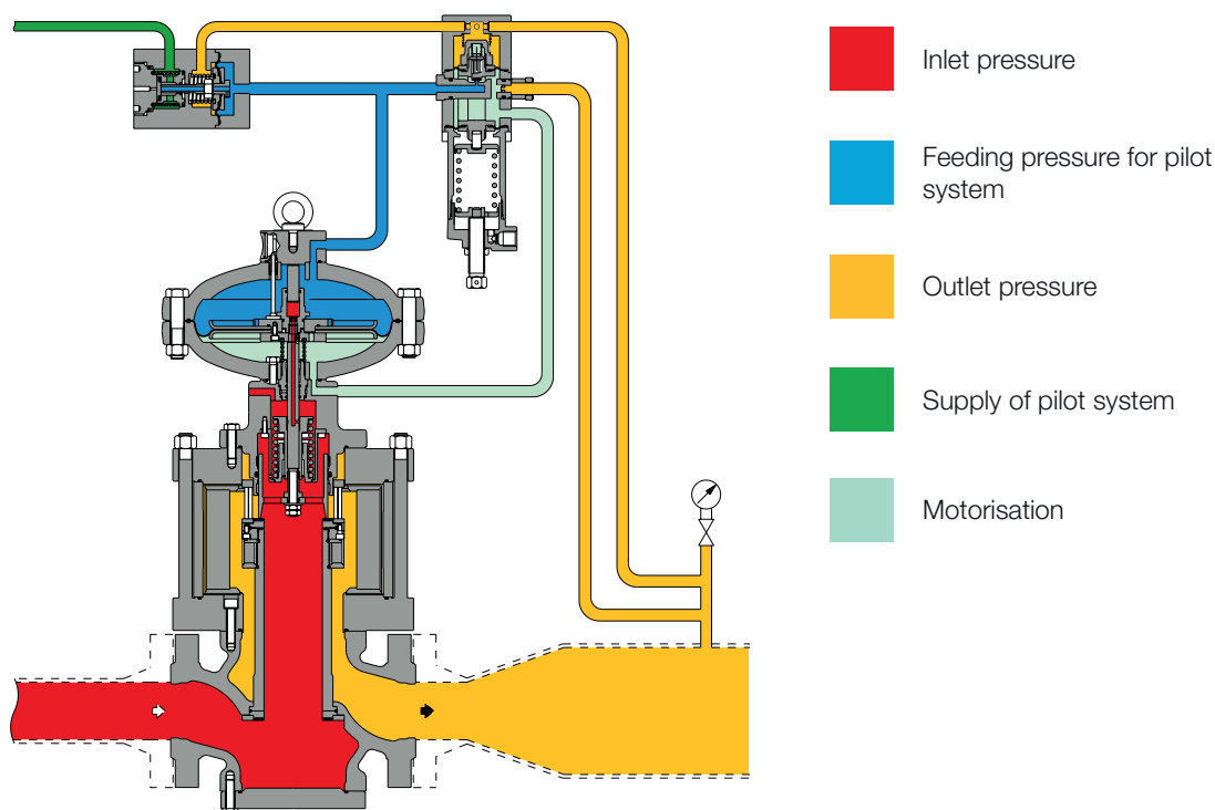
Figure 7 Reflux 819/FO with DB/819 silencer
