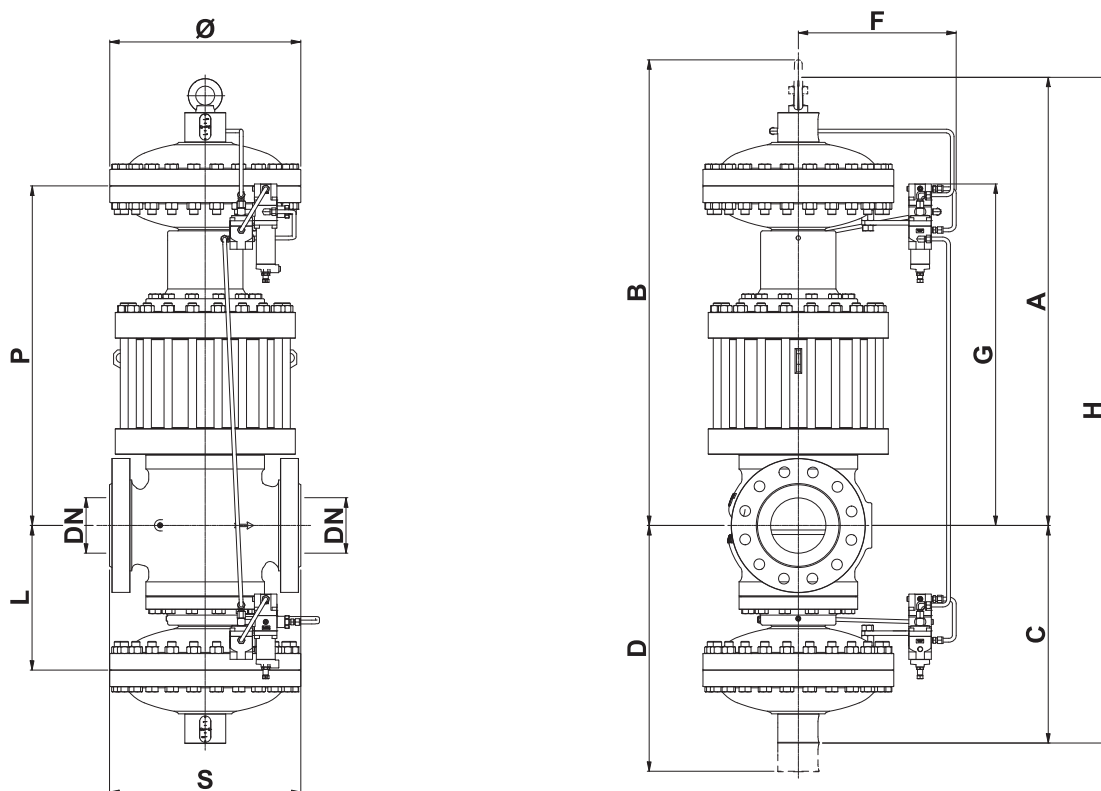
Figure 16 Dimensions du Reflux 819/FO + DB/819 + PM/819
