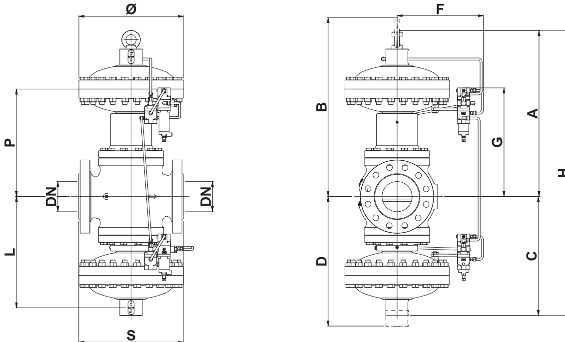
Figure 13 Dimensions du Reflux 819/FO + PM/819
