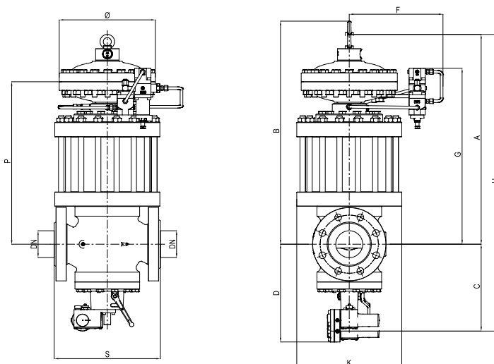
Figure 15 Reflux 819 + DB/819 + SB/82 or HB/97 dimensions
