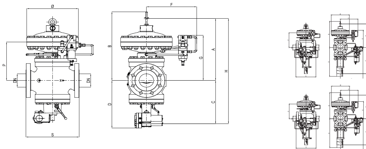
Figure 12 Reflux 819 + SB/82 or HB/97 dimensions
