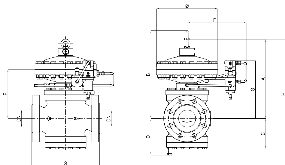
Figure 11 Reflux 819 dimensions
