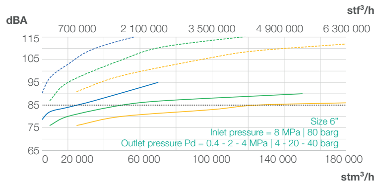
Chart 1 Reflux 819's silencer efficiency charts
