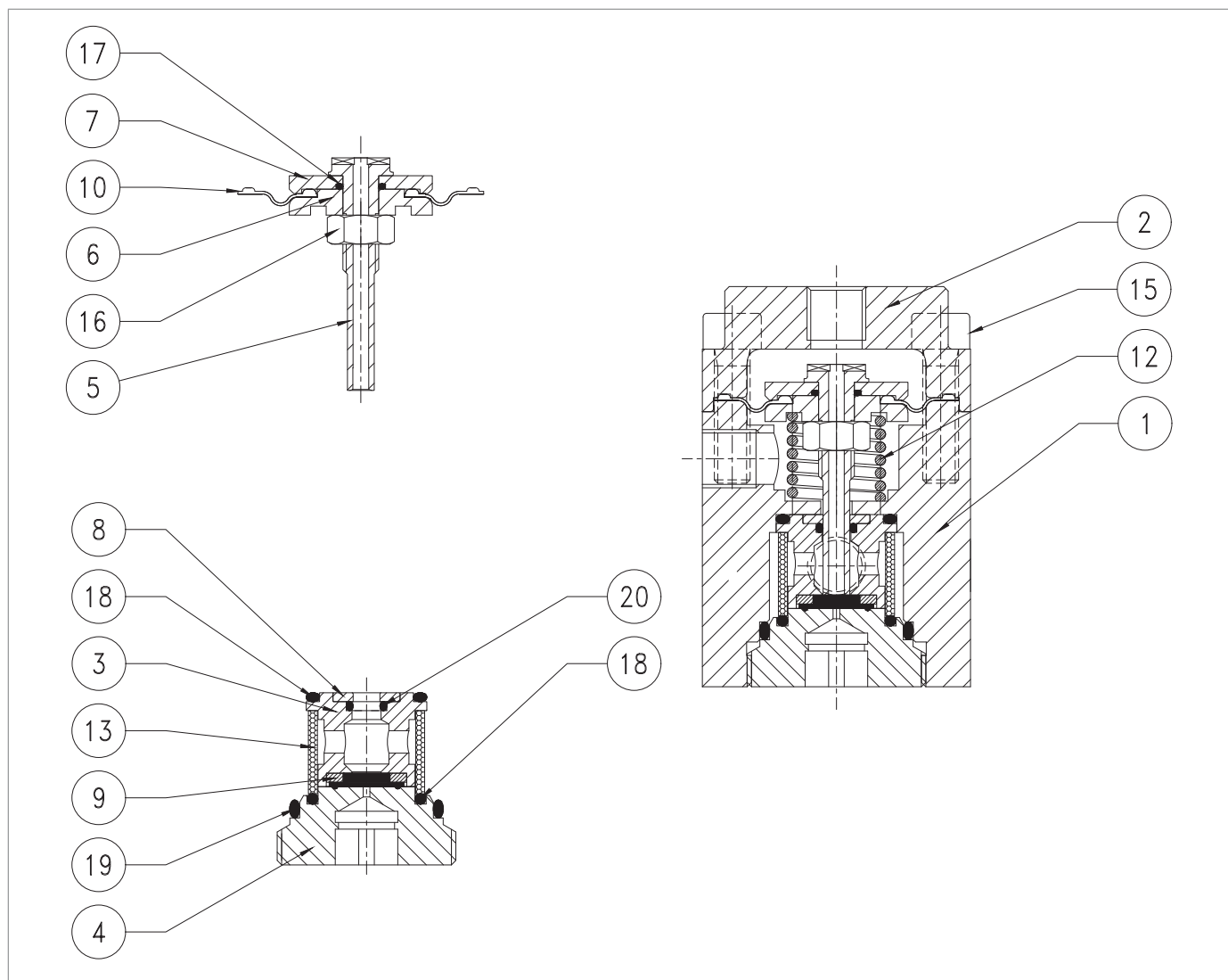
Prereducator R14/A
