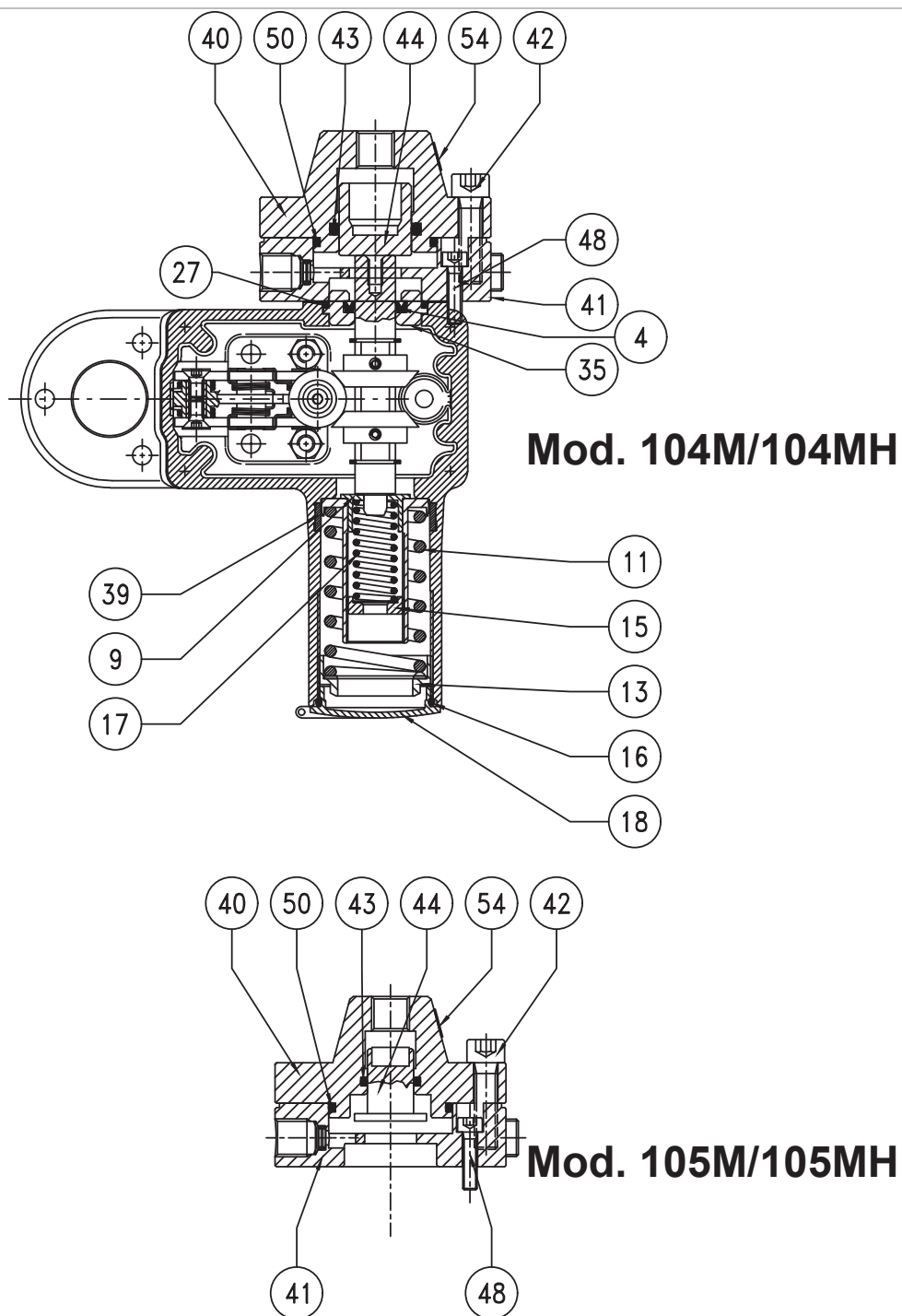
Fig. 9.77. Presostato Mod. 104M/104MH ÷ 105M/105MH
