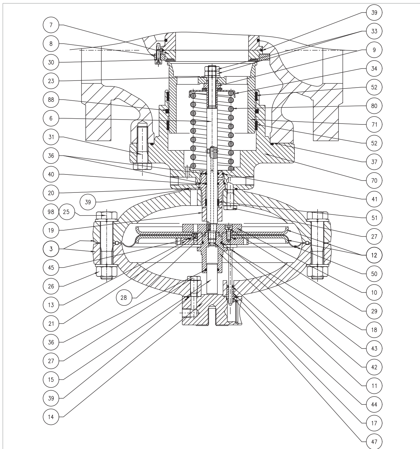
Fig. 9.62. Monitor incorporado PM/819 3"÷ 4"
