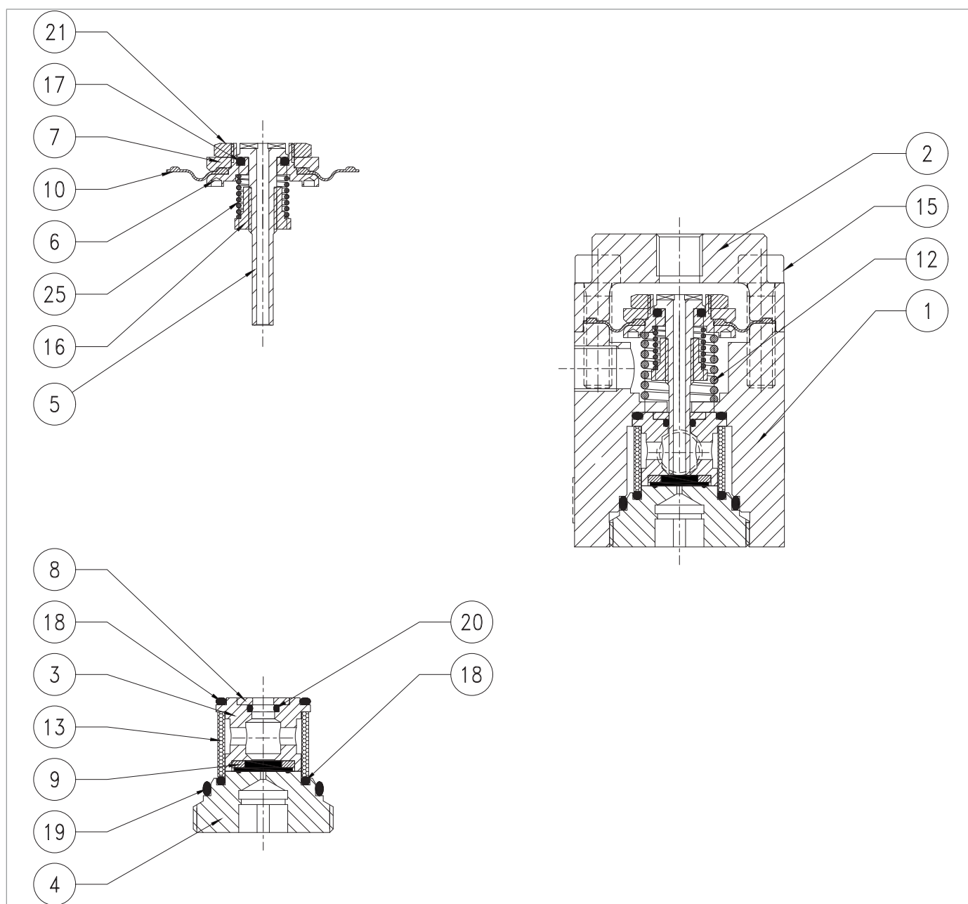
Fig. 9.67. Prerreductor R14/A/ FO
