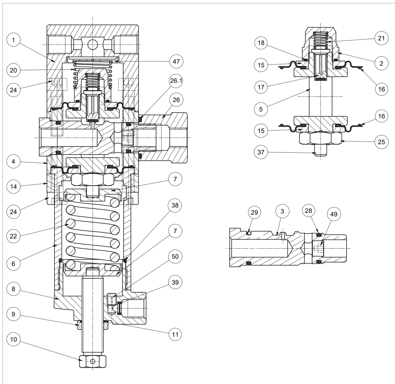
Piloto 204/A/FO-204/A y 205/A/FO-205/A
