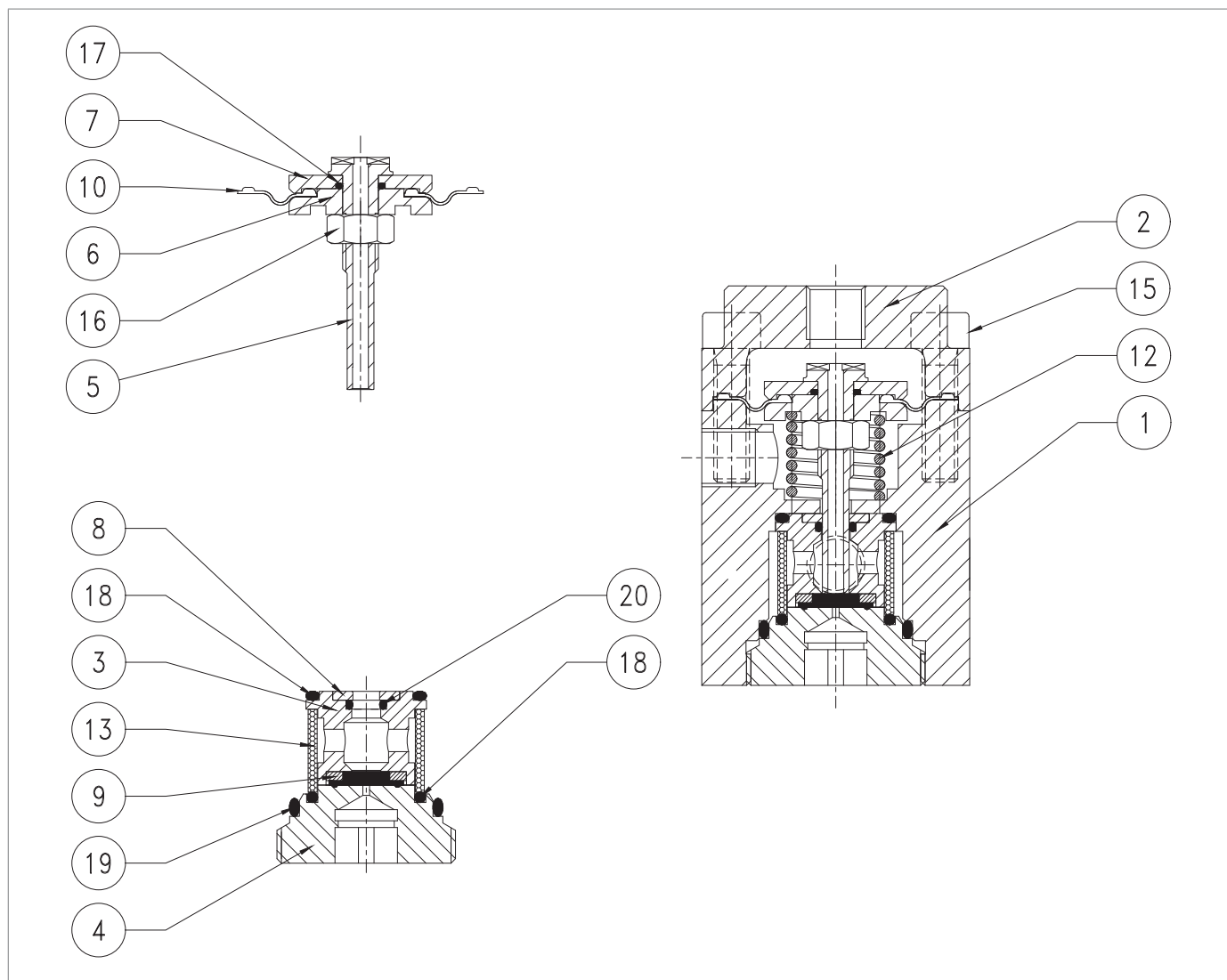
Fig. 9.68. Prerreductor R14/A
