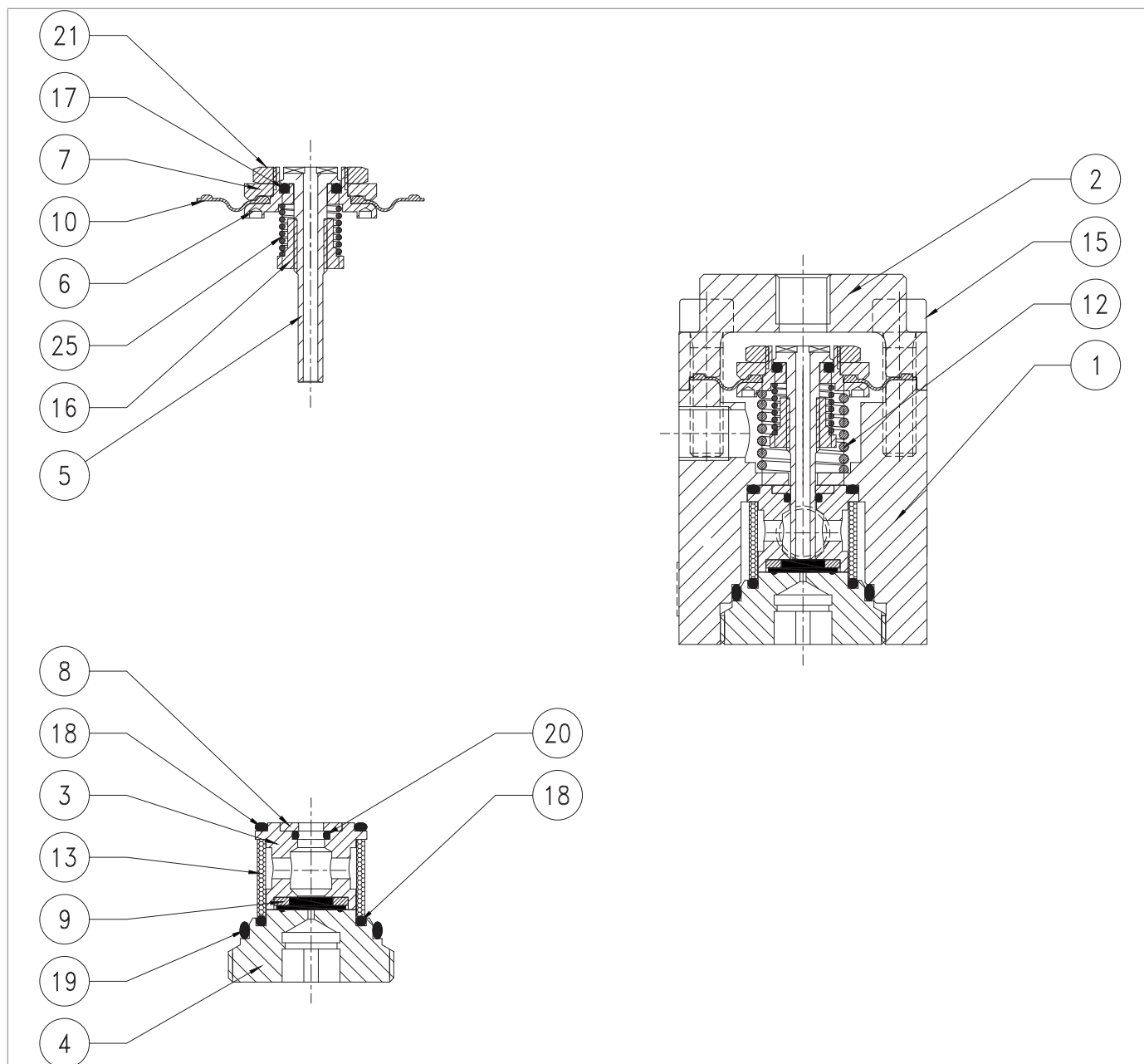
Prereducator R14/A/ FO
