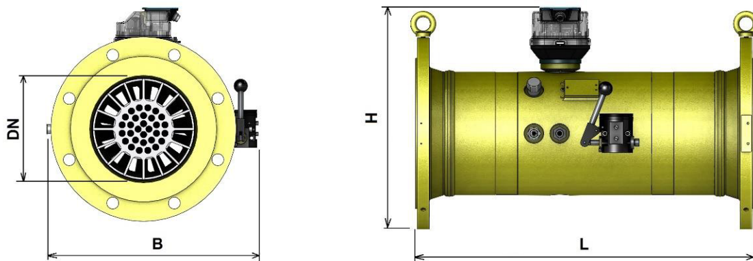
Figure 16 iM-TM steel body dimensions
