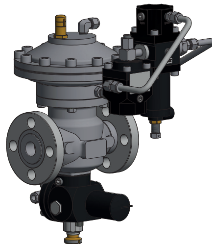
Figure 4 Dixi AP with SB/87 slam shut
