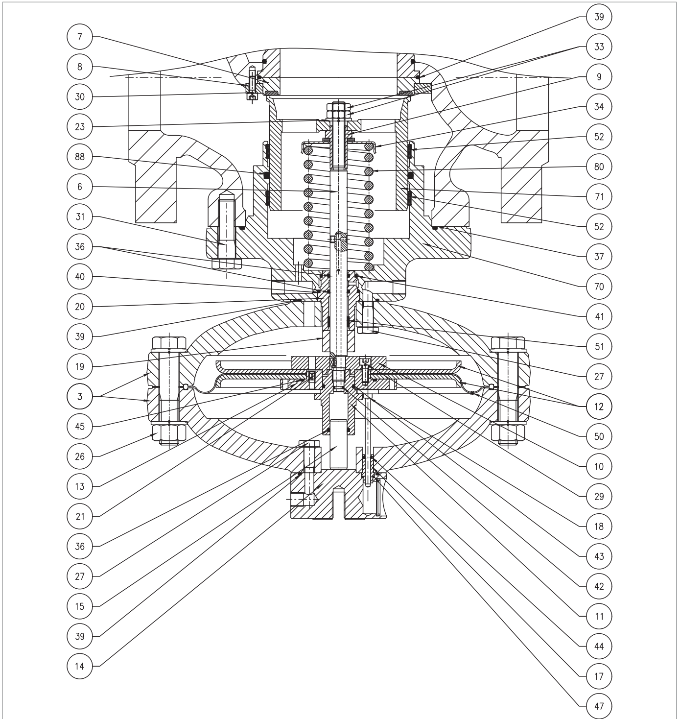
Monitor incorporado PM/819 3" ÷ 4"
