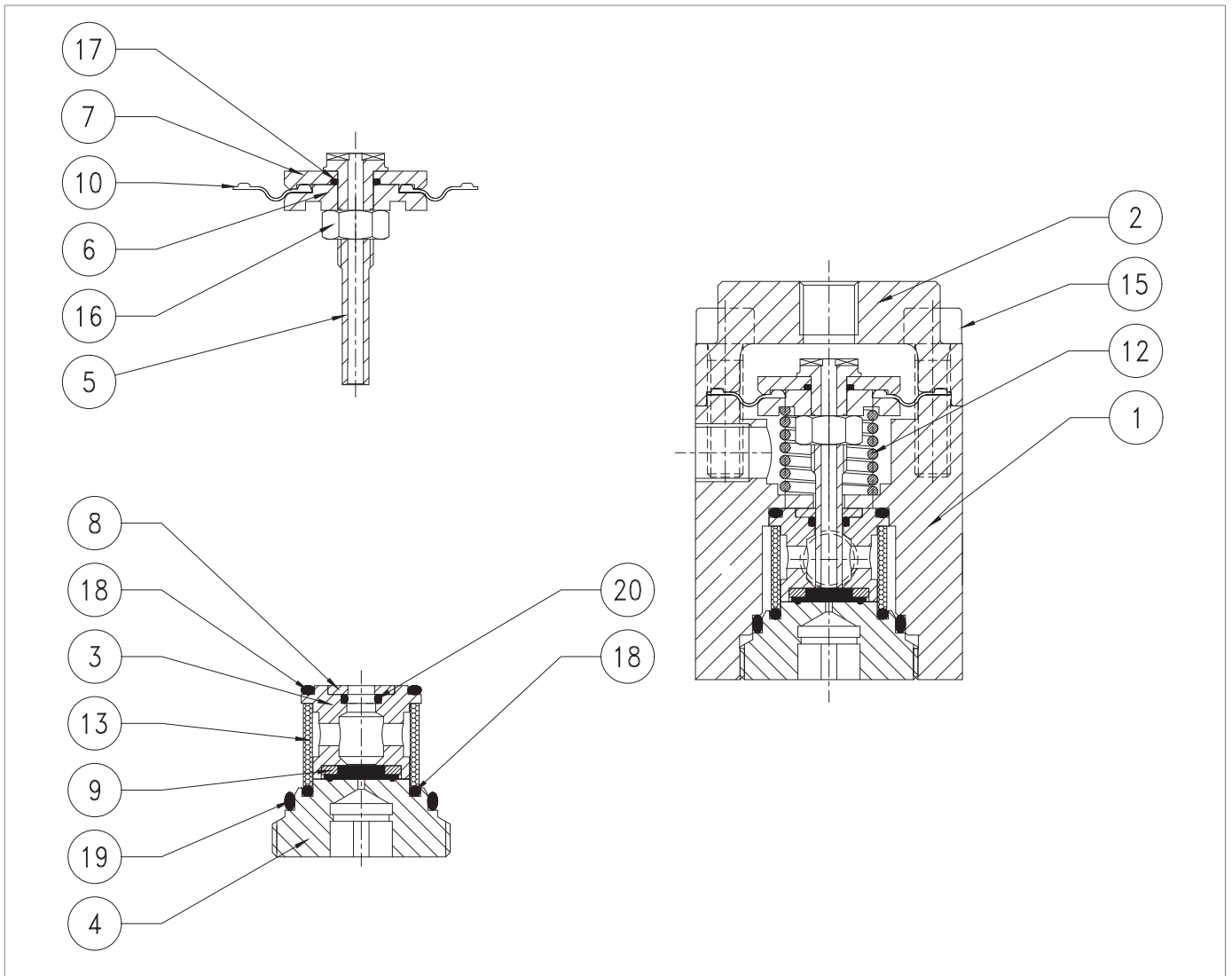
Fig. 9.68. Pre-reductor R14/A
