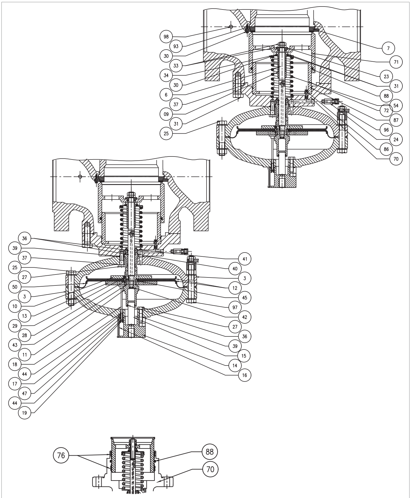
Fig. 9.63. Monitor incorporado PM/819 6"÷ 10"
