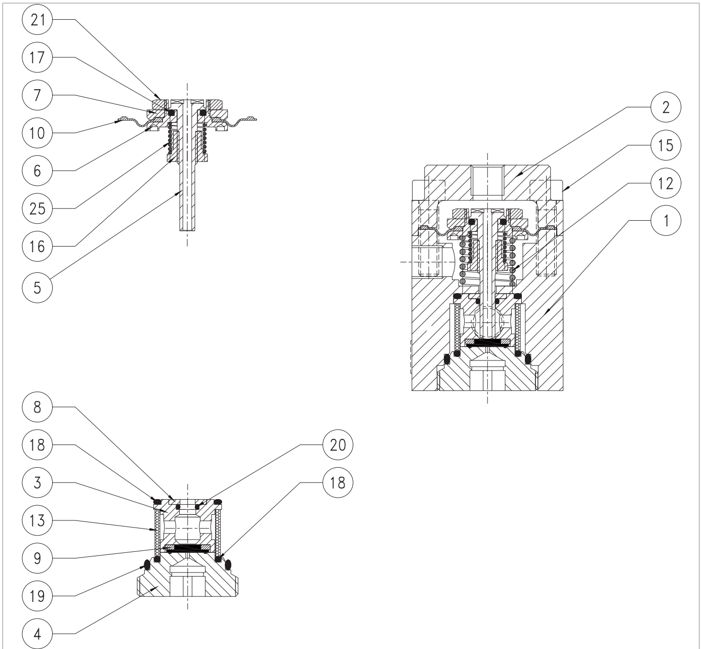
Fig. 9.67. Prerreductor R14/A/FO
