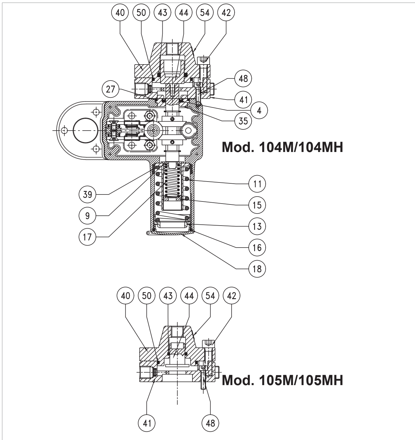
Fig. 9.77. Presostato Mod. 104M/104MH ÷ 105M/105MH
