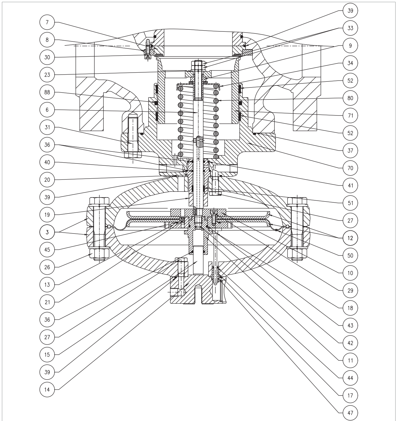
Fig. 9.62. Monitor incorporado PM/819 3"÷ 4"
