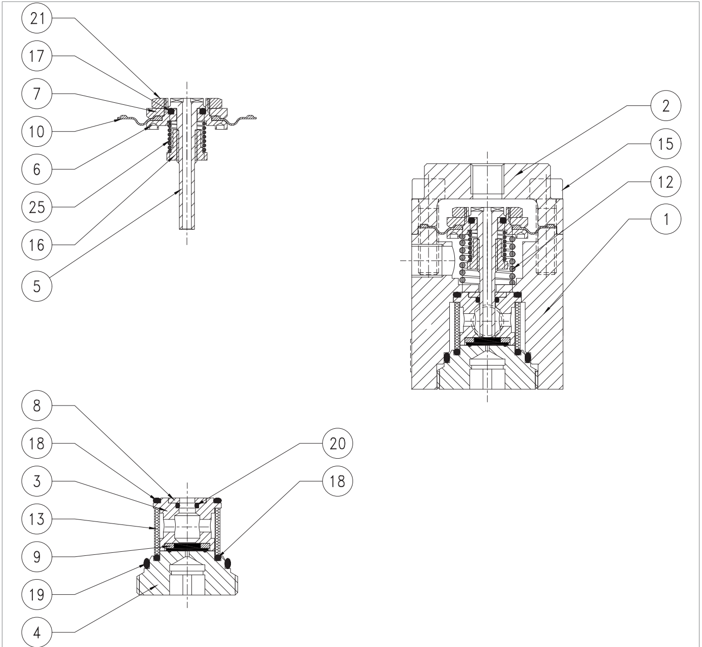
Prerreductor R14/A/FO
