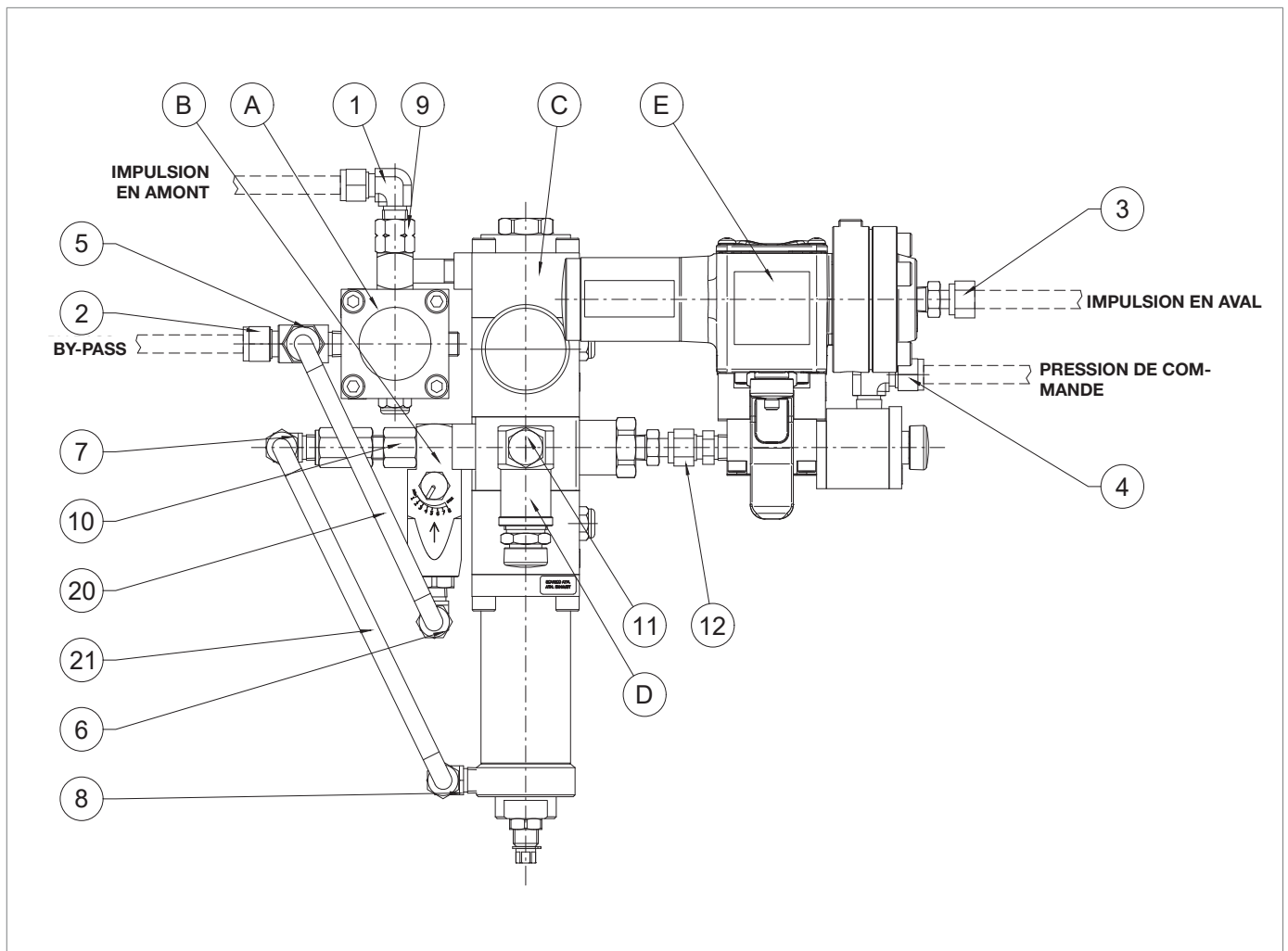
Fig. 9.32. LINE OFF 2.0
